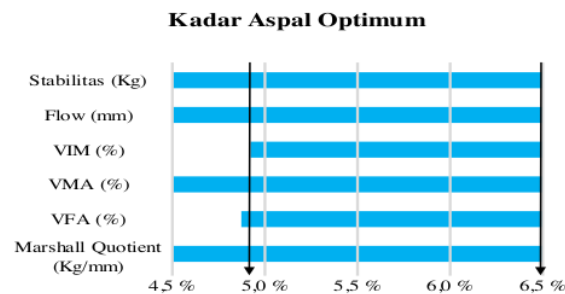
Gambar 4.5 Diagram penentuan kadar aspal optimum
