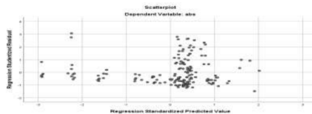
Gambar 3 Scatterplot
