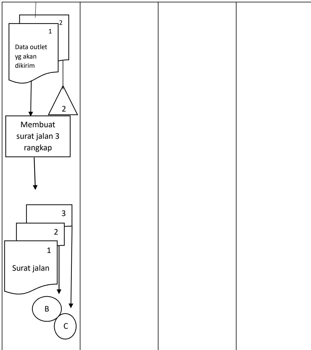
Gambar 3.5 Flowchart Persediaan
